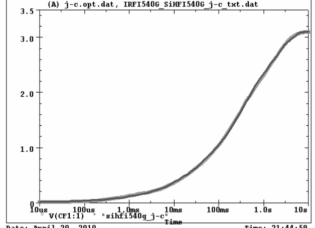
SiHFI540G Filter j-c Temperature: 27.0
