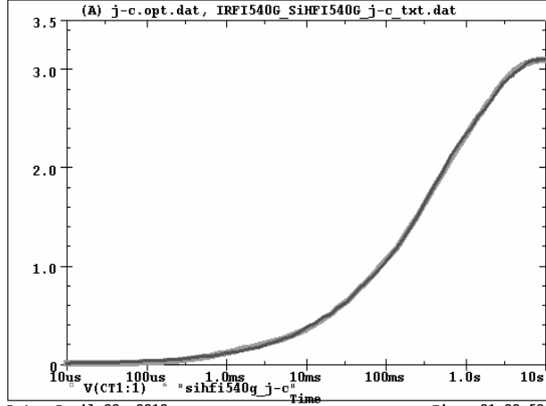
SiHFI540G Tank j-c Temperature: 27.0
